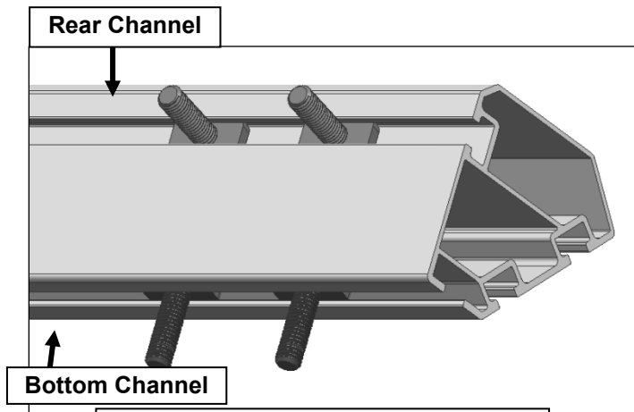
(Fig 10) Insert T-bolts into the rear and bottom channels on the universal mounting tube.
