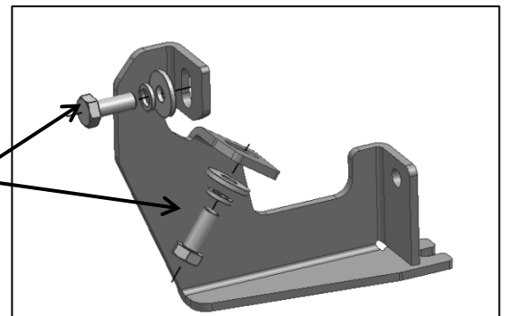
(Fig 4) Attach (2) Center/Rear Mounting Brackets to the center and rear locations
