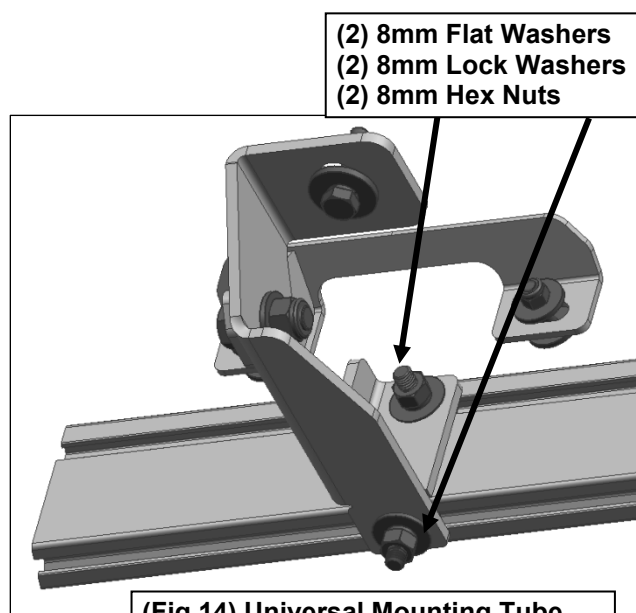
(Fig 14) Universal Mounting Tube attached to the Mounting Bracket.
