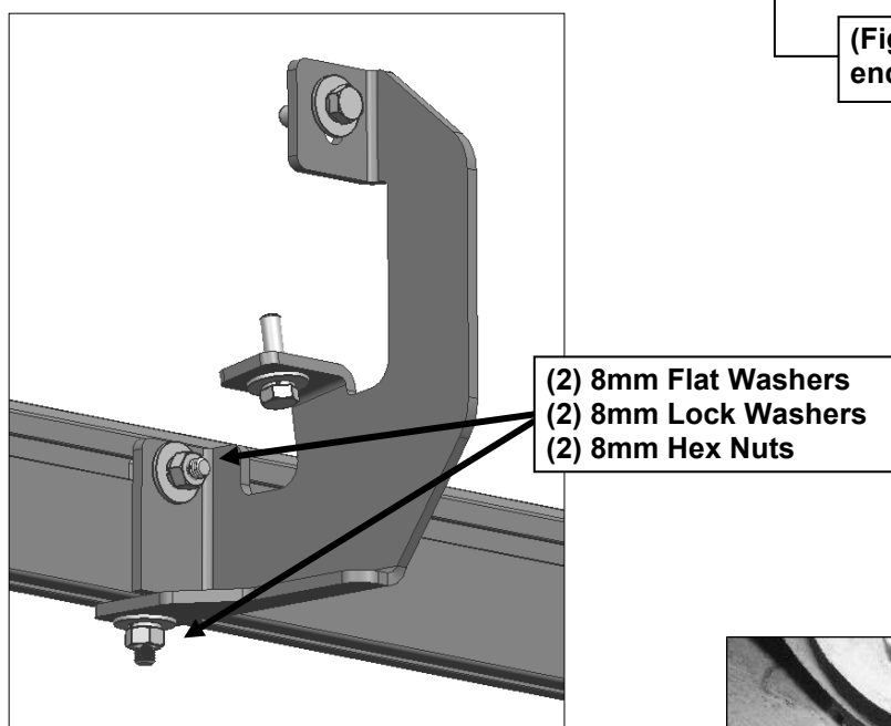
(Fig 13) Attach the Universal Mounting Tube to the Mounting Brackets.
