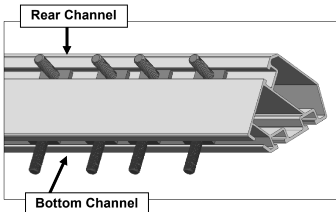
(Fig 6) Insert T-bolts into the rear and bottom channels on the universal mounting tube.
