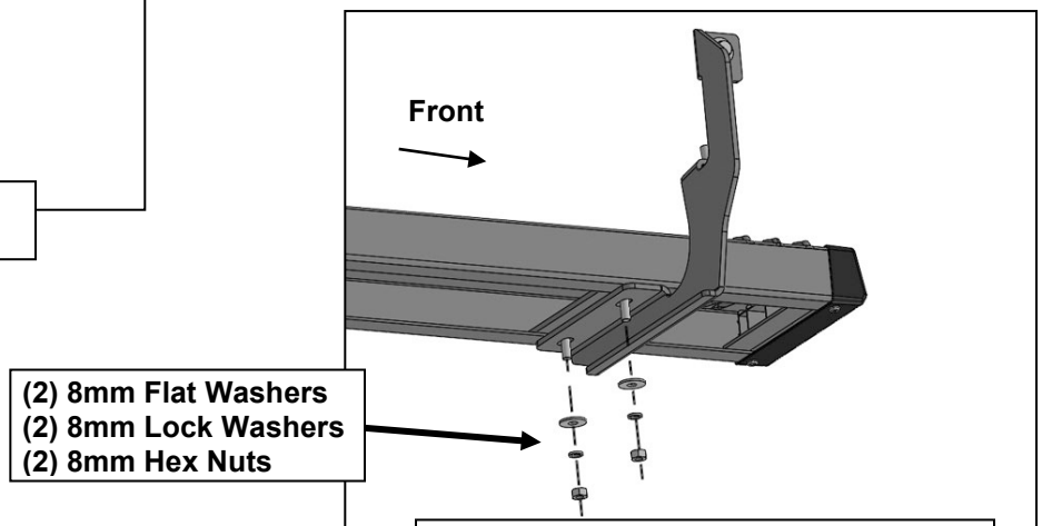
(Fig 8) Running Board attached to Driver/left side front Mounting Bracket
