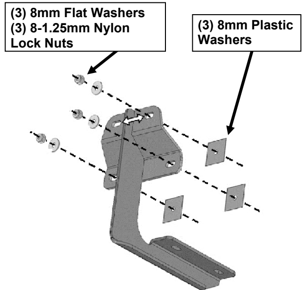
(Fig 4) Typical Bracket installation
