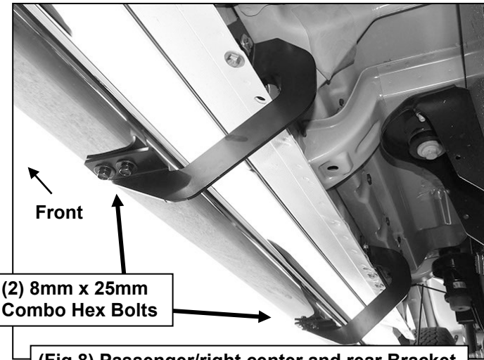
(Fig 8) Passenger/right center and rear Bracket
