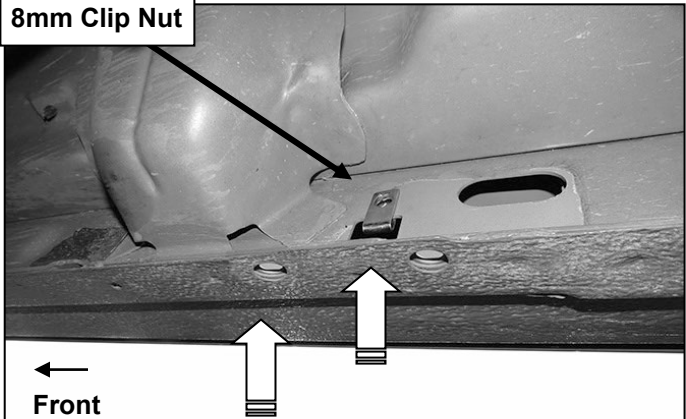
(Fig 5) Passenger/right center mounting location
