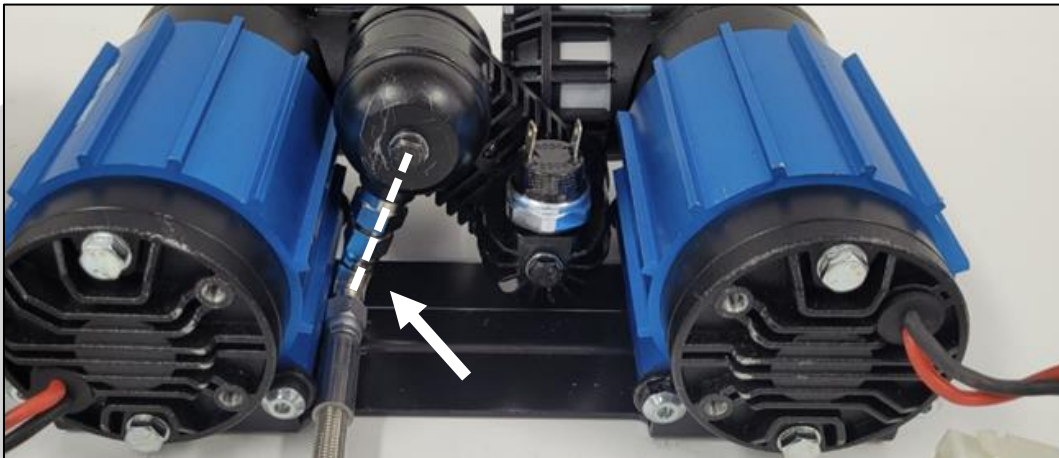
Figure 7. Positioning of the reinforced air line by manifold cap rotation
