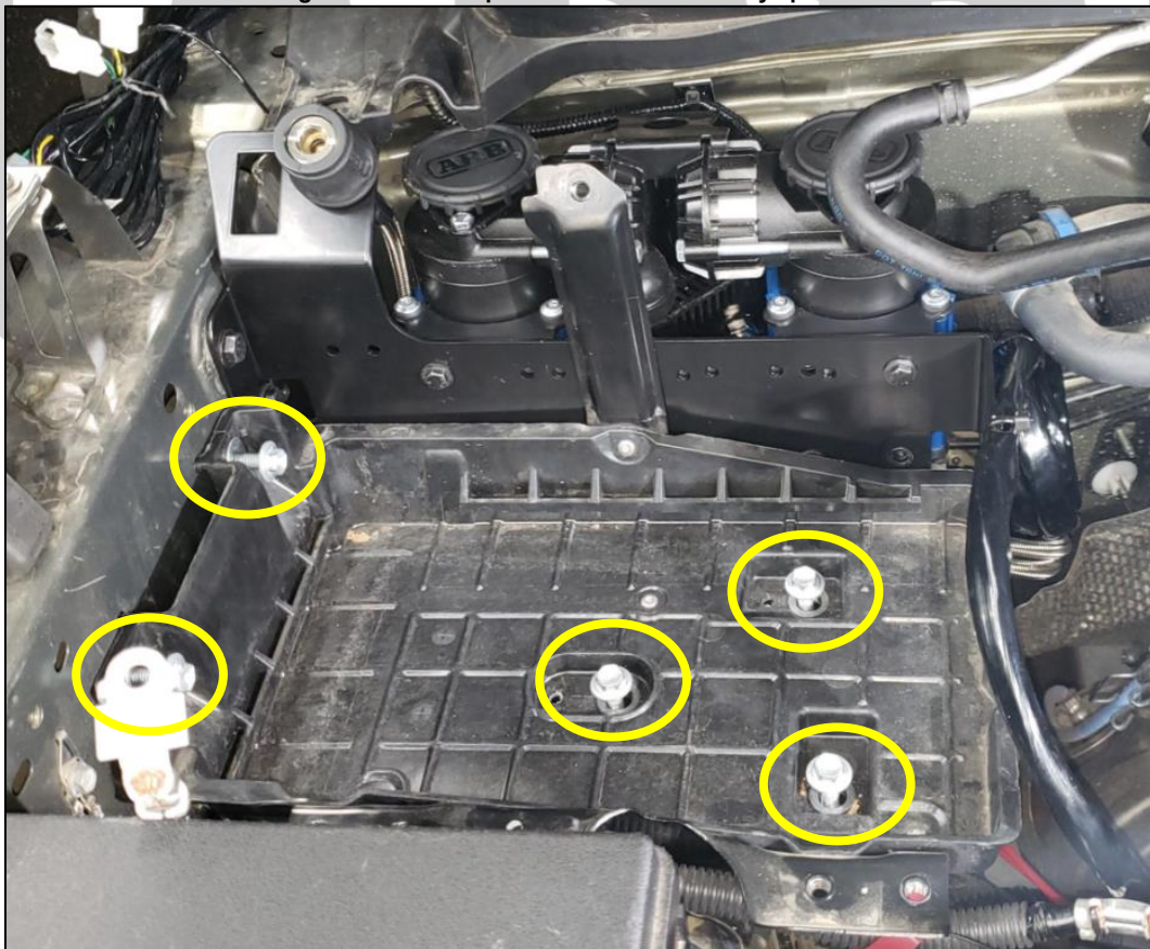
Figure 19. Battery tray and original fasteners
