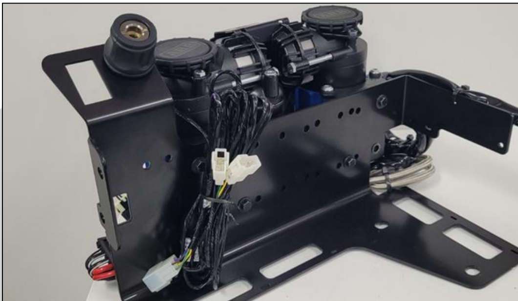
Figure 9. Compressor bracket assembly ready for installation into a vehicle
