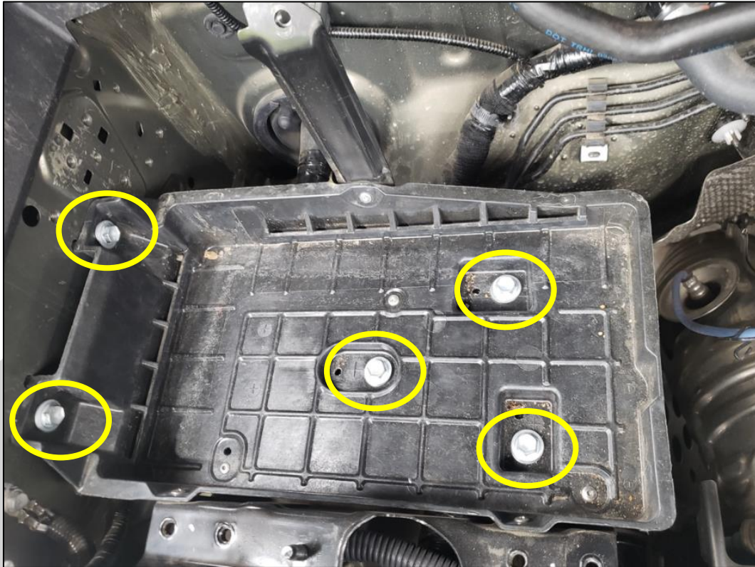
Figure 13. Battery tray and original fasteners
