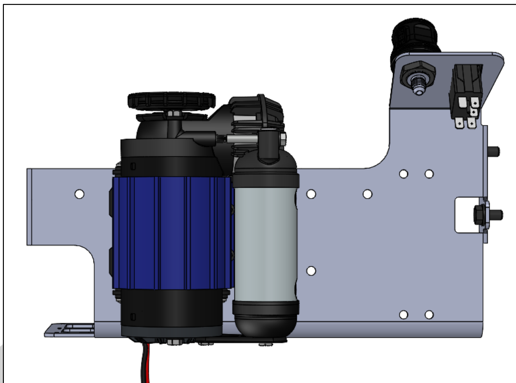
Figure 3. Single Compressor bracket pre-assembly rear view
