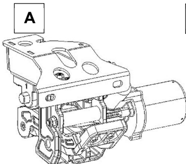
Driver Front Bracket Assembly
