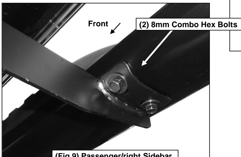
(Fig 9) Passenger/right Sidebar attached to Bracket pictured
